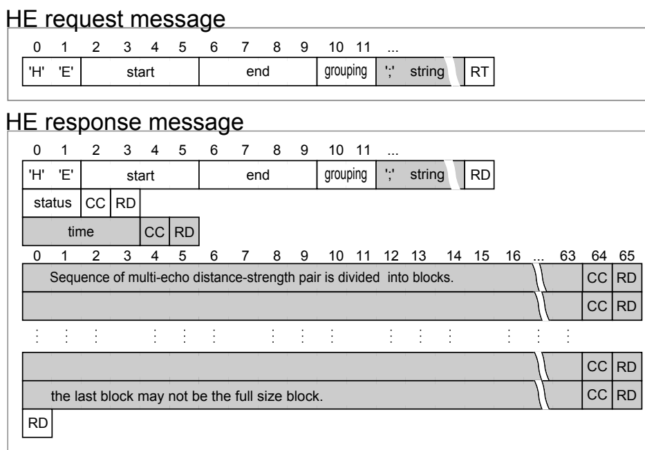
Figure 15: HE Message Format
