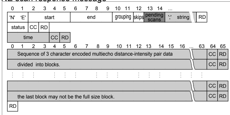
Figure 19: NE Message Format
