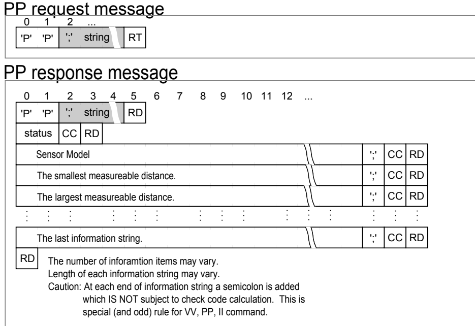
Figure 29: PP Message Format
