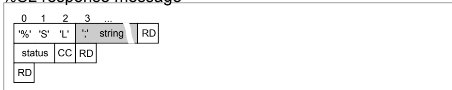
Figure 23: %SL Message Format
