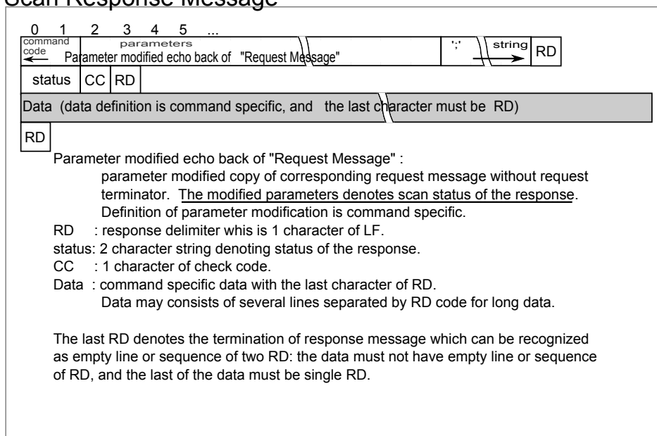
Figure 4: Scan Response Message Format
