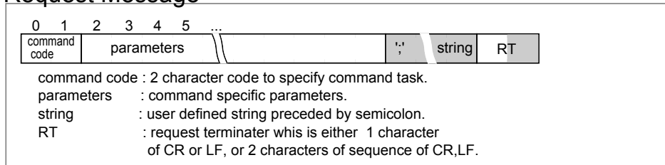
Figure 1: Request Message Format
