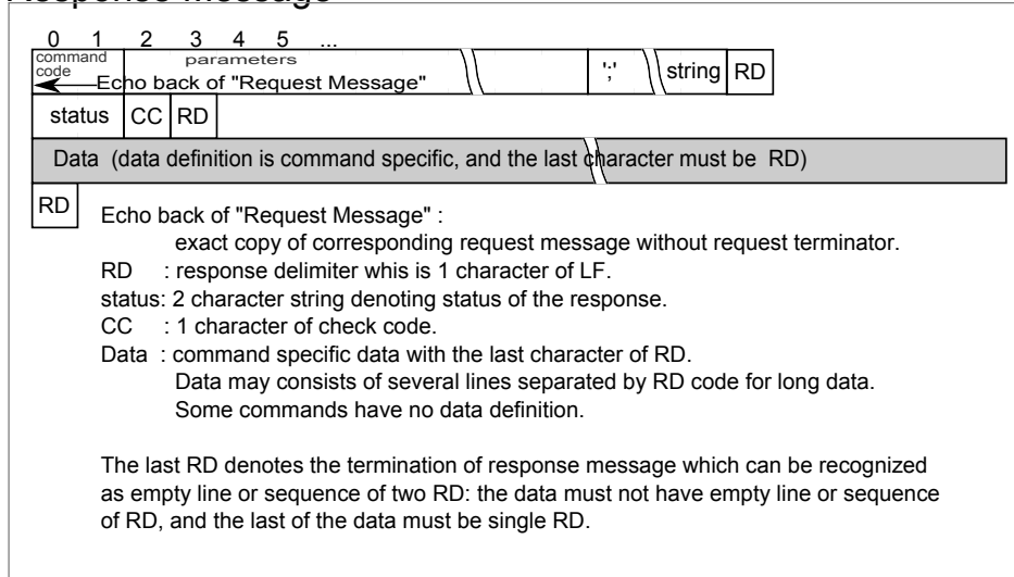
Figure 3: Response Message Format
