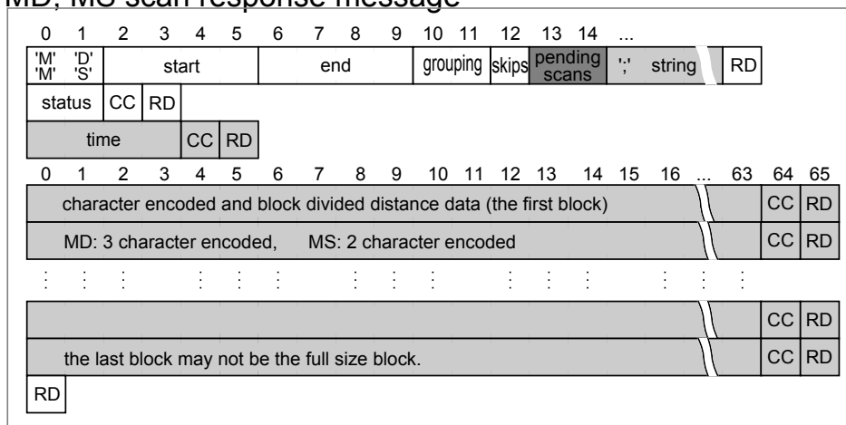
Figure 16: MD, MS Message Format
