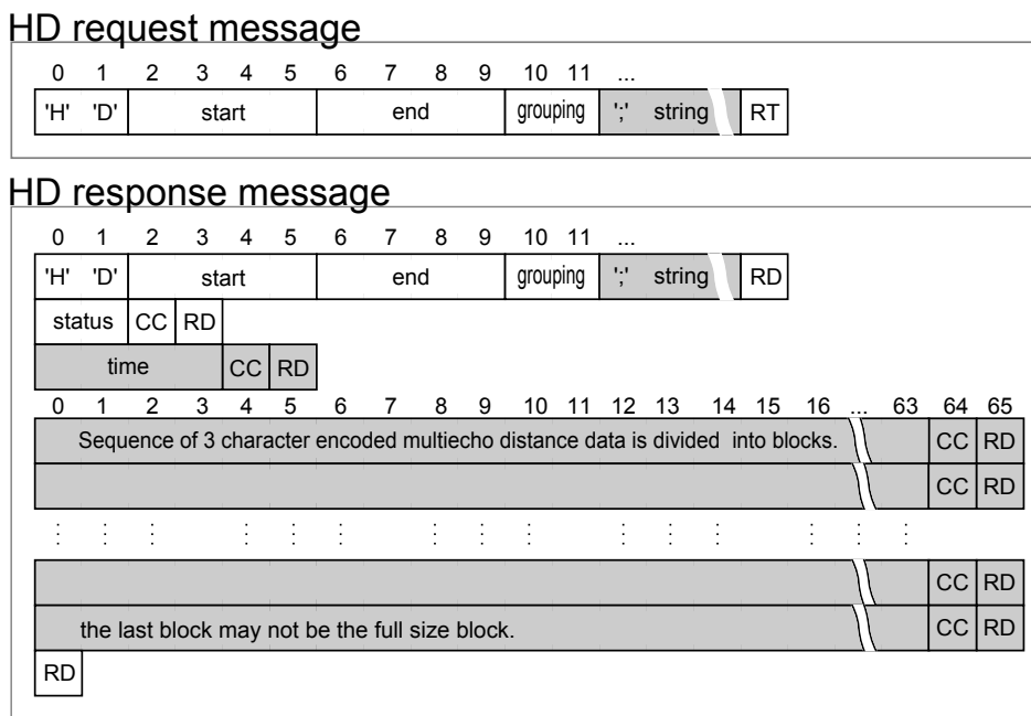
Figure 14: HD Message Format
