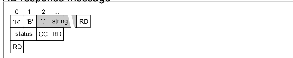
Figure 26: RB Message Format
