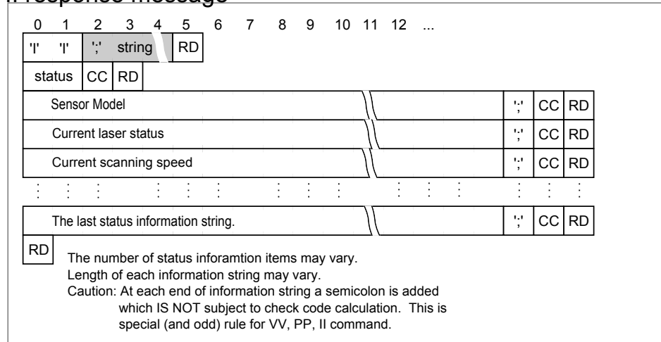
Figure 30: II Message Format
