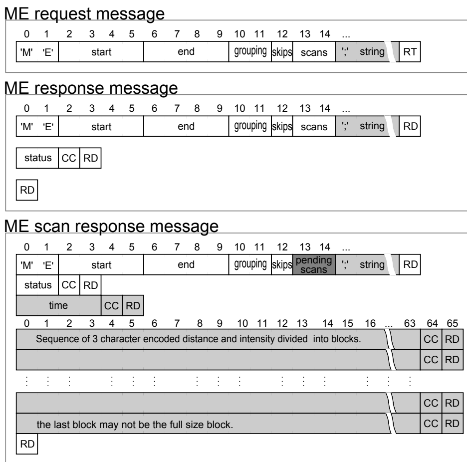
Figure 17: ME Message Format
